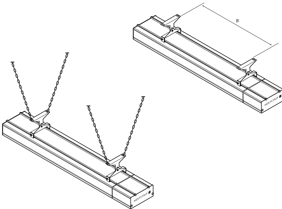
Right: Surface Mounting, using the standard mounting brackets.
